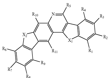
Formula 2C
