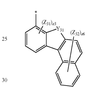
Formula 6-12
